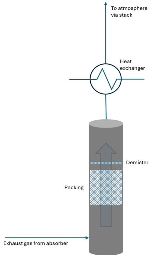
Figure 5- Diagrammatic representation of scrubber
