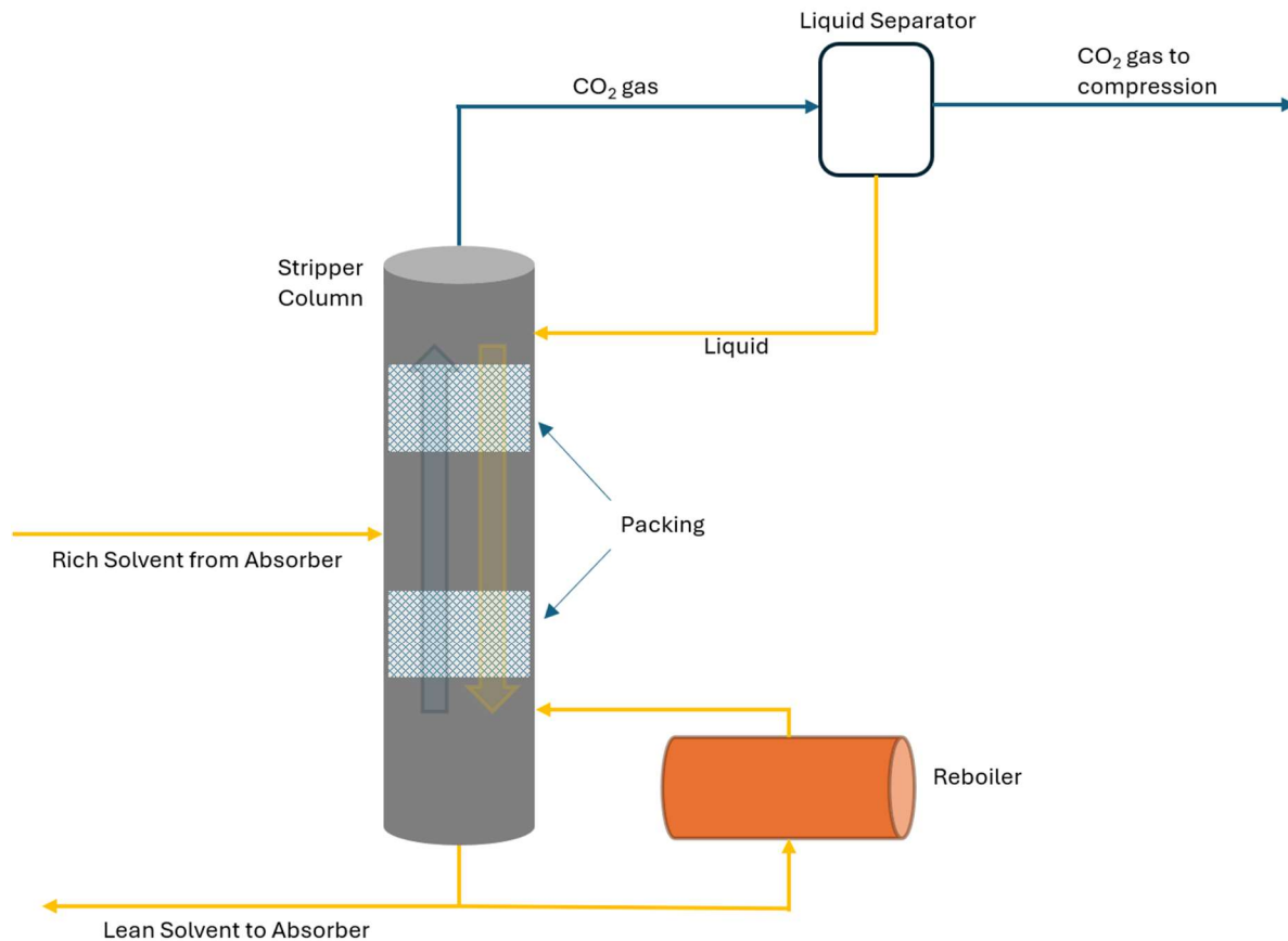
Figure 6 – Diagrammatic representation of stripper / reboiler
